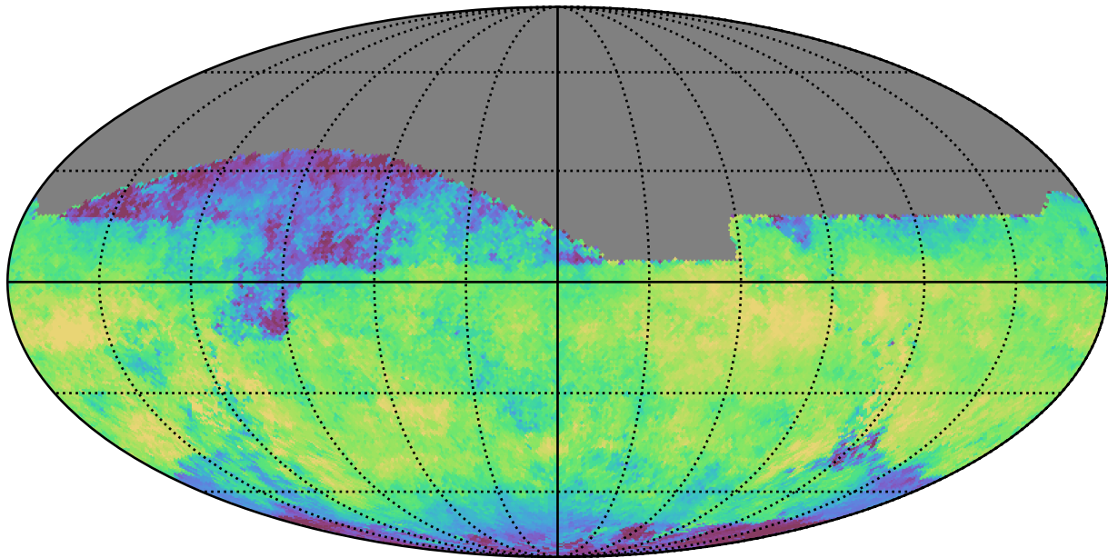
ddf_loaded_half_fl2_v3.4_10yrs All sky i band: Median skyBrightness
