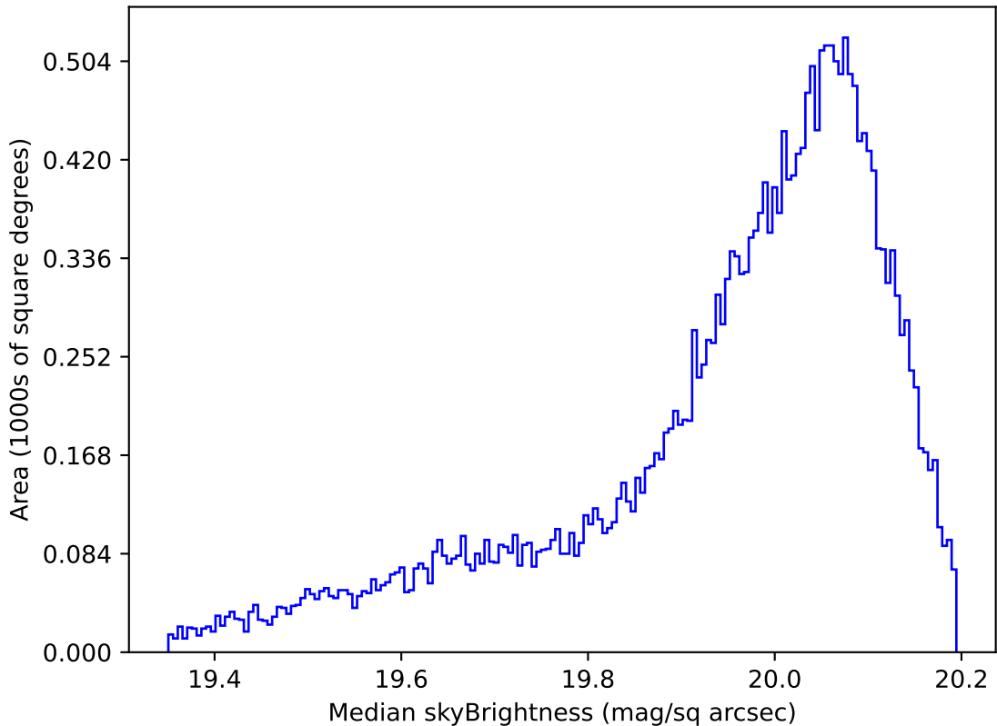
ddf_loaded_half_fl2_v3.4_10yrs All sky i band: Median skyBrightness
