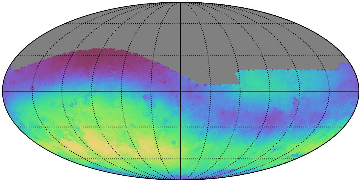
ddf_loaded_half_fl2_v3.4_10yrs All sky g band: Median skyBrightness
