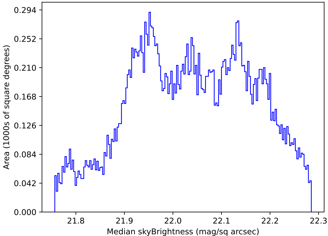
ddf_loaded_half_fl2_v3.4_10yrs All sky g band: Median skyBrightness
