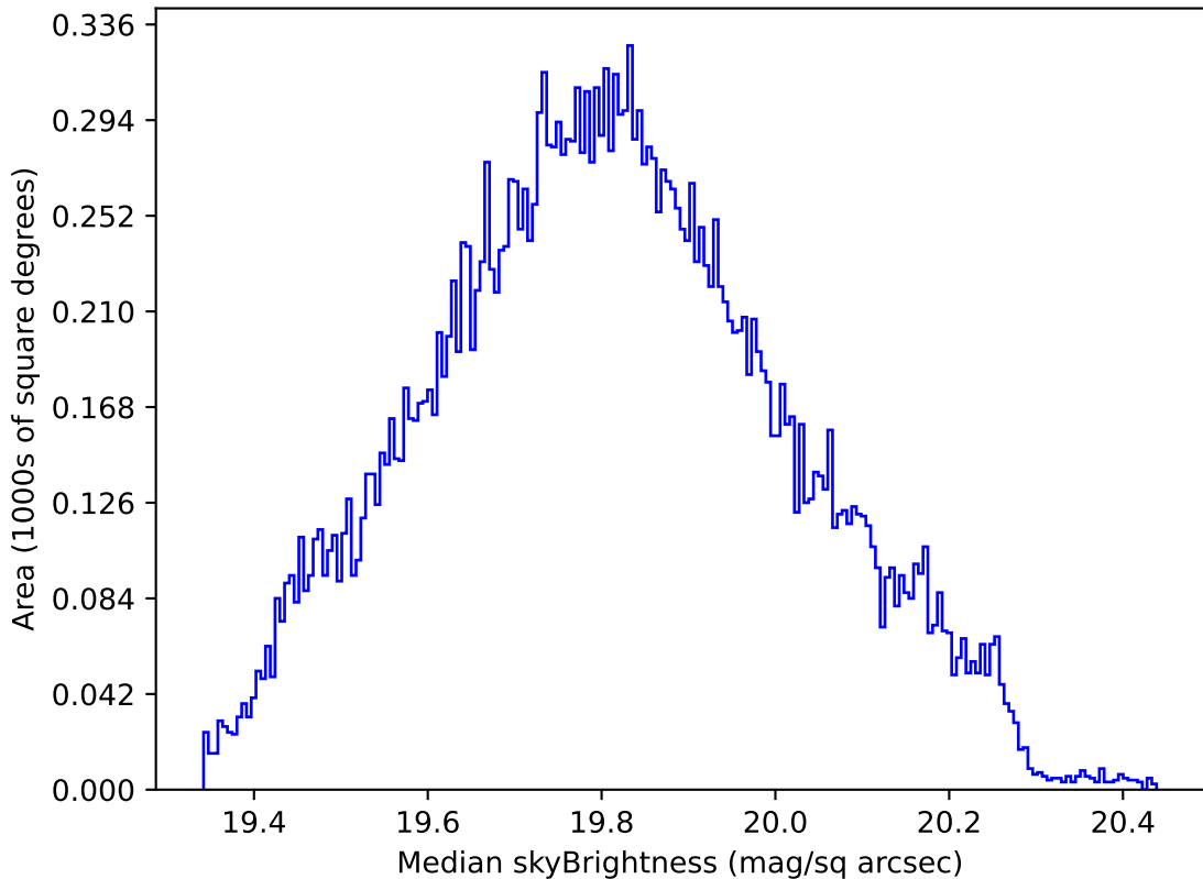
ddf_loaded_half_fl2_v3.4_10yrs All sky all bands: Median skyBrightness
