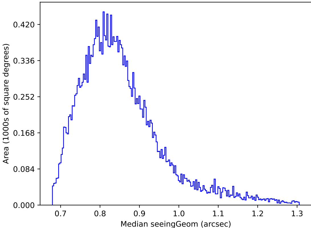
ddf_loaded_half_fl2_v3.4_10yrs Yr 1 z band: Median seeingGeom
