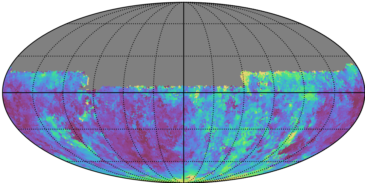
ddf_loaded_half_fl2_v3.4_10yrs Yr 1 y band: Median seeingGeom
