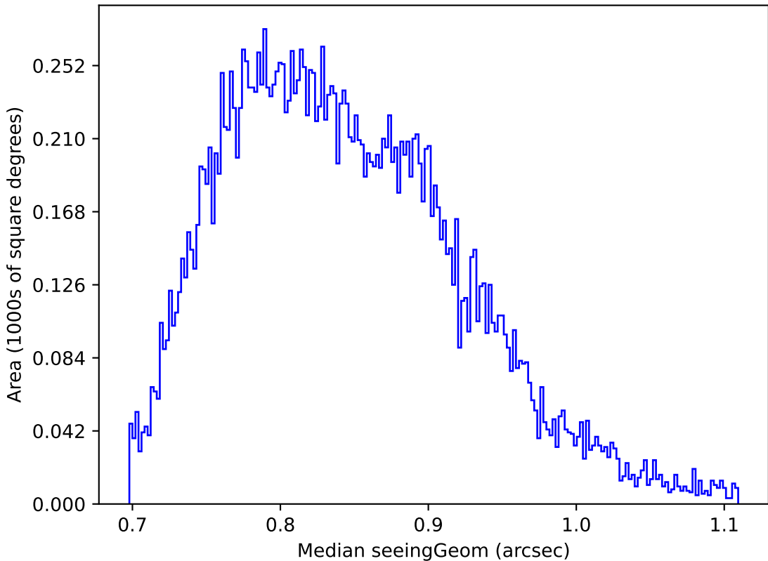
ddf_loaded_half_fl2_v3.4_10yrs Yr 1 y band: Median seeingGeom
