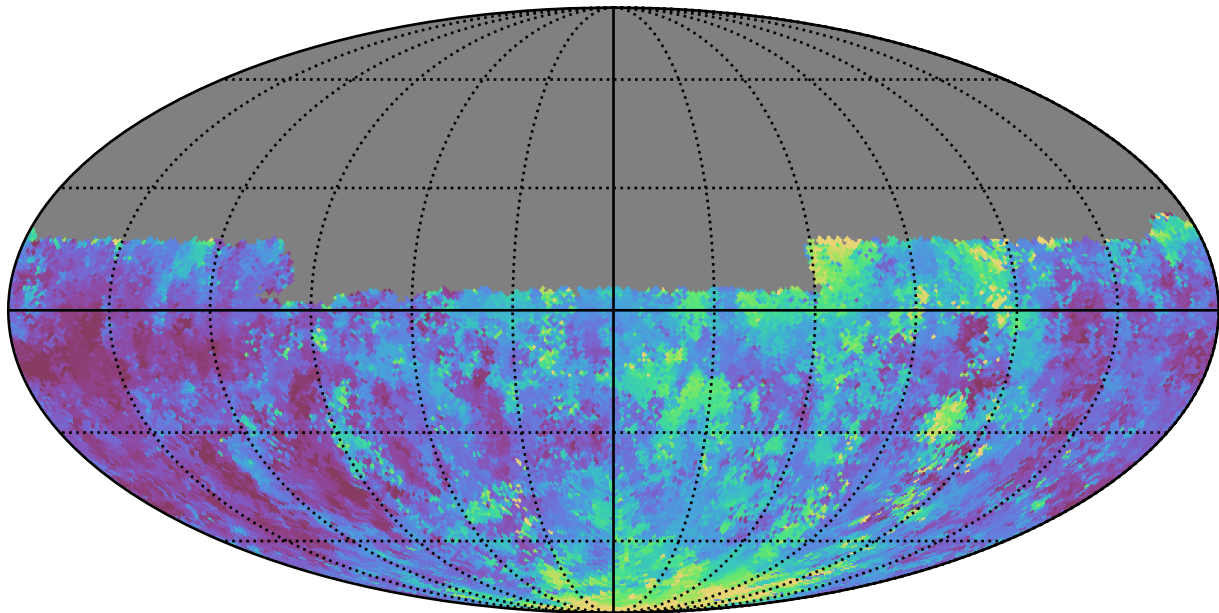
ddf_loaded_half_fl2_v3.4_10yrs Yr 1 u band: Median seeingGeom
