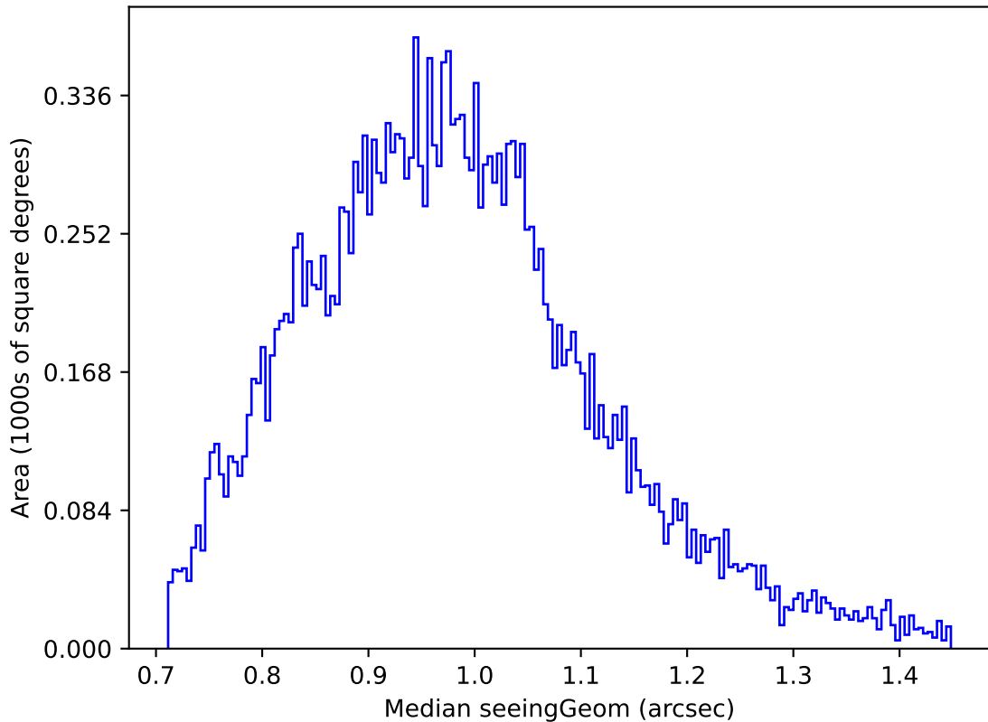
ddf_loaded_half_fl2_v3.4_10yrs Yr 1 u band: Median seeingGeom
