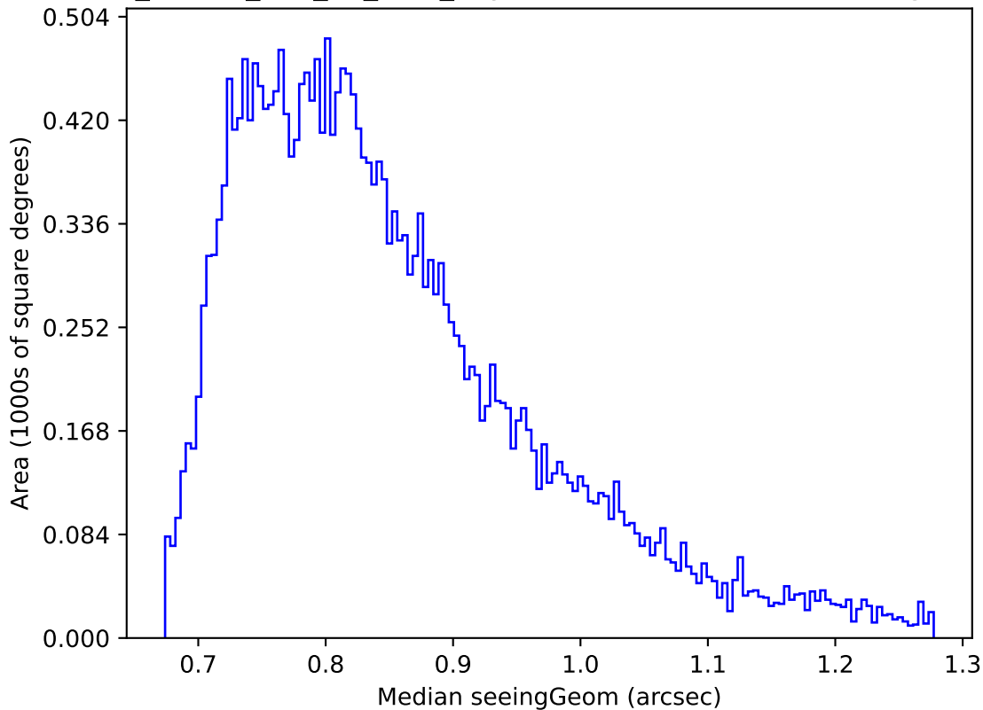
ddf_loaded_half_fl2_v3.4_10yrs Yr 1 r band: Median seeingGeom
