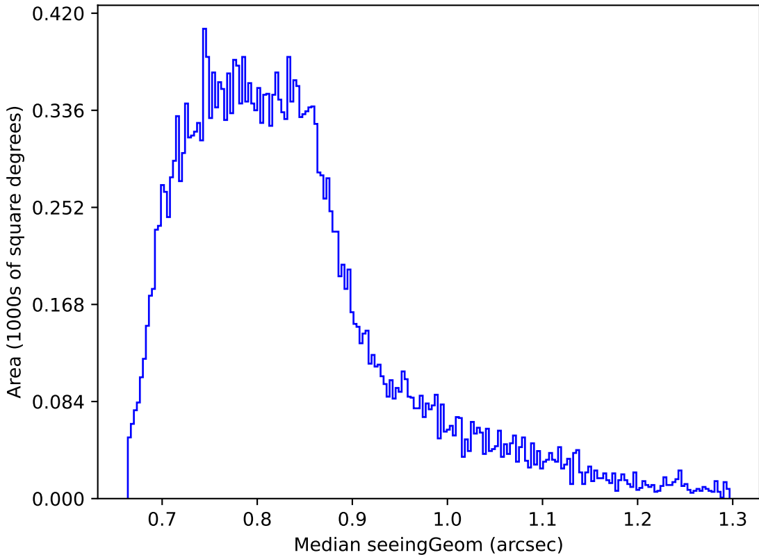
ddf_loaded_half_fl2_v3.4_10yrs Yr 1 i band: Median seeingGeom
