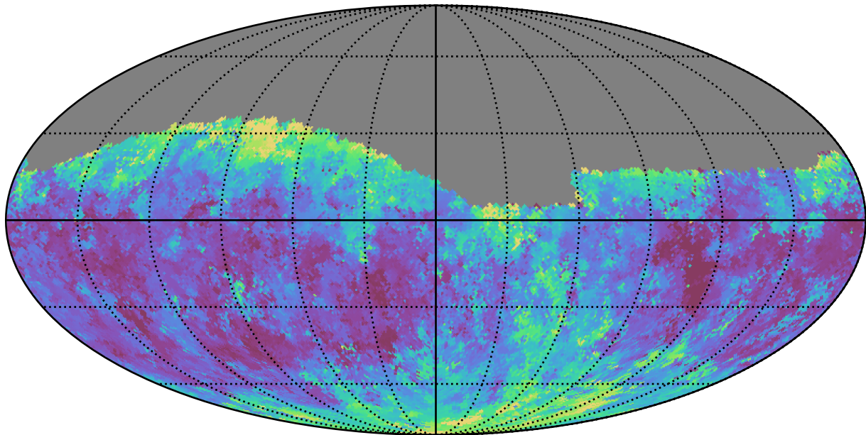
ddf_loaded_half_fl2_v3.4_10yrs Yr 1 g band: Median seeingGeom
