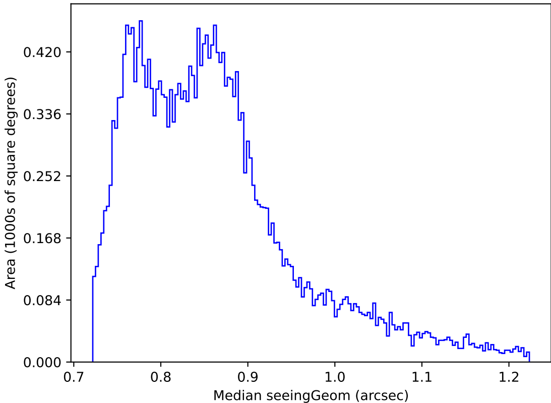
ddf_loaded_half_fl2_v3.4_10yrs Yr 1 all bands: Median seeingGeom
