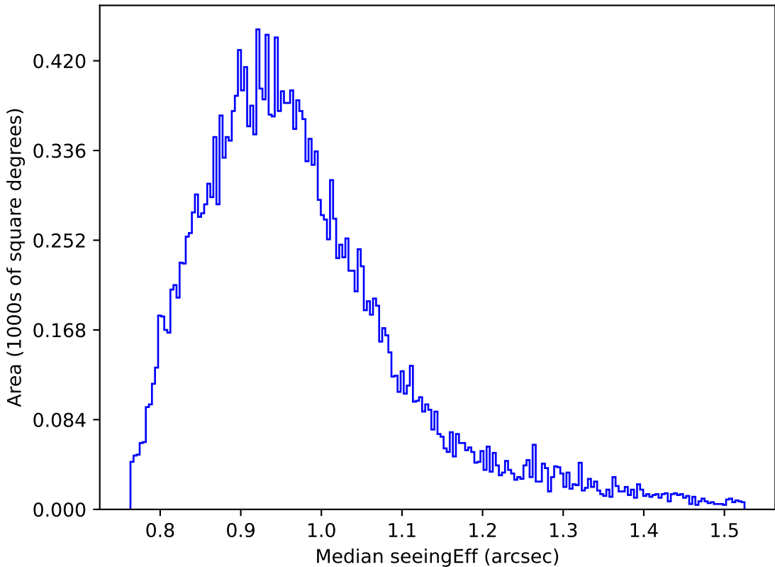
ddf_loaded_half_fl2_v3.4_10yrs Yr 1 z band: Median seeingEff
