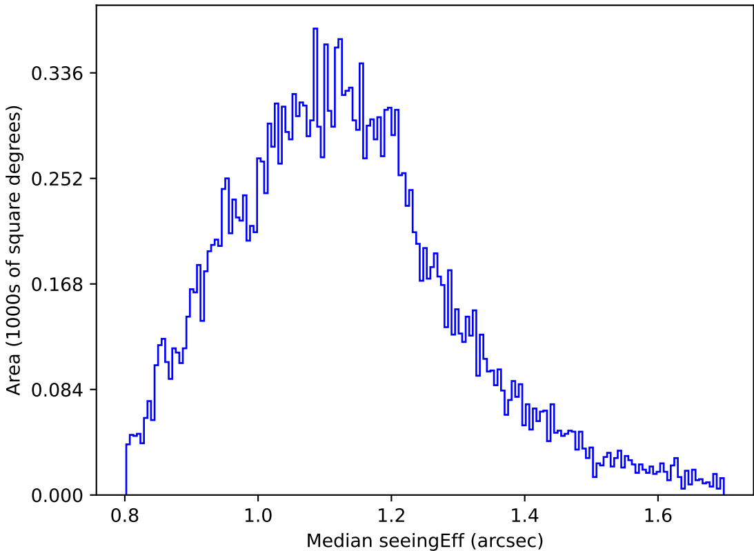
ddf_loaded_half_fl2_v3.4_10yrs Yr 1 u band: Median seeingEff
