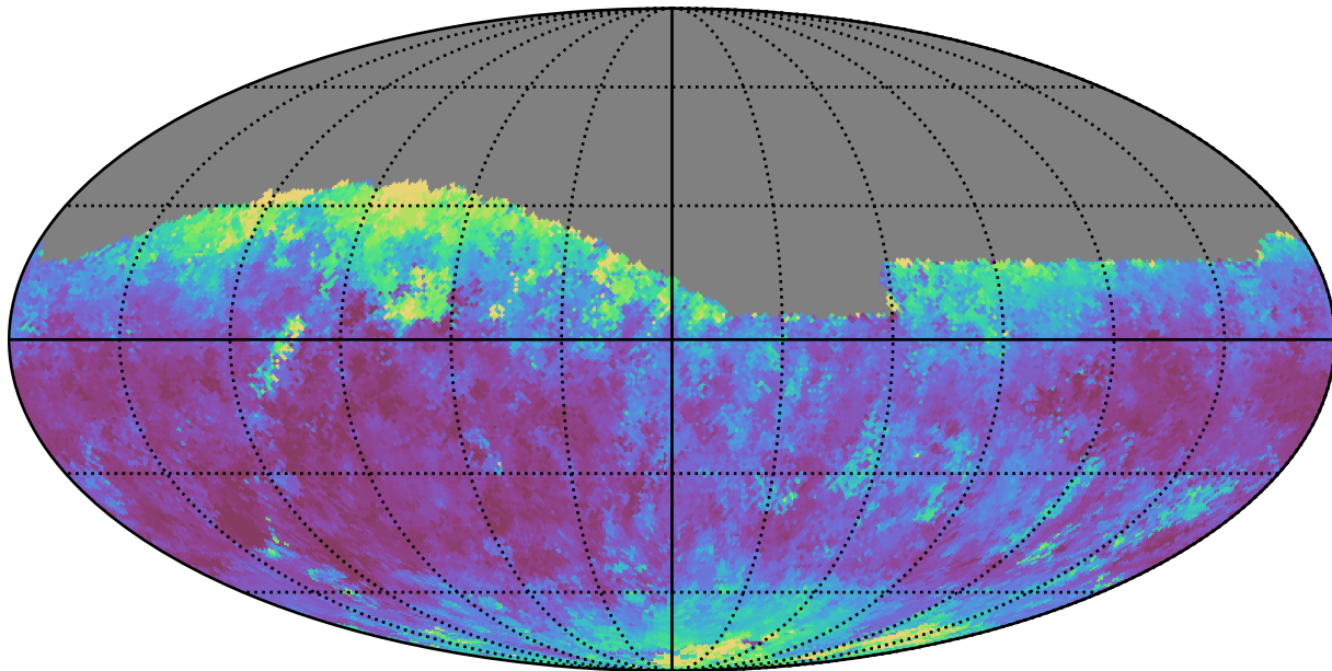
ddf_loaded_half_f12_v3.4_10yrs Yr 1 r band: Median seeingEff
