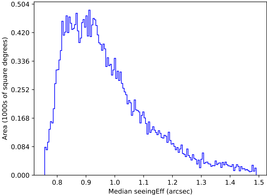
ddf_loaded_half_fl2_v3.4_10yrs Yr 1 r band: Median seeingEff
