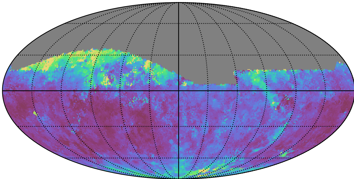
ddf_loaded_half_f12_v3.4_10yrs Yr 1 i band: Median seeingEff
