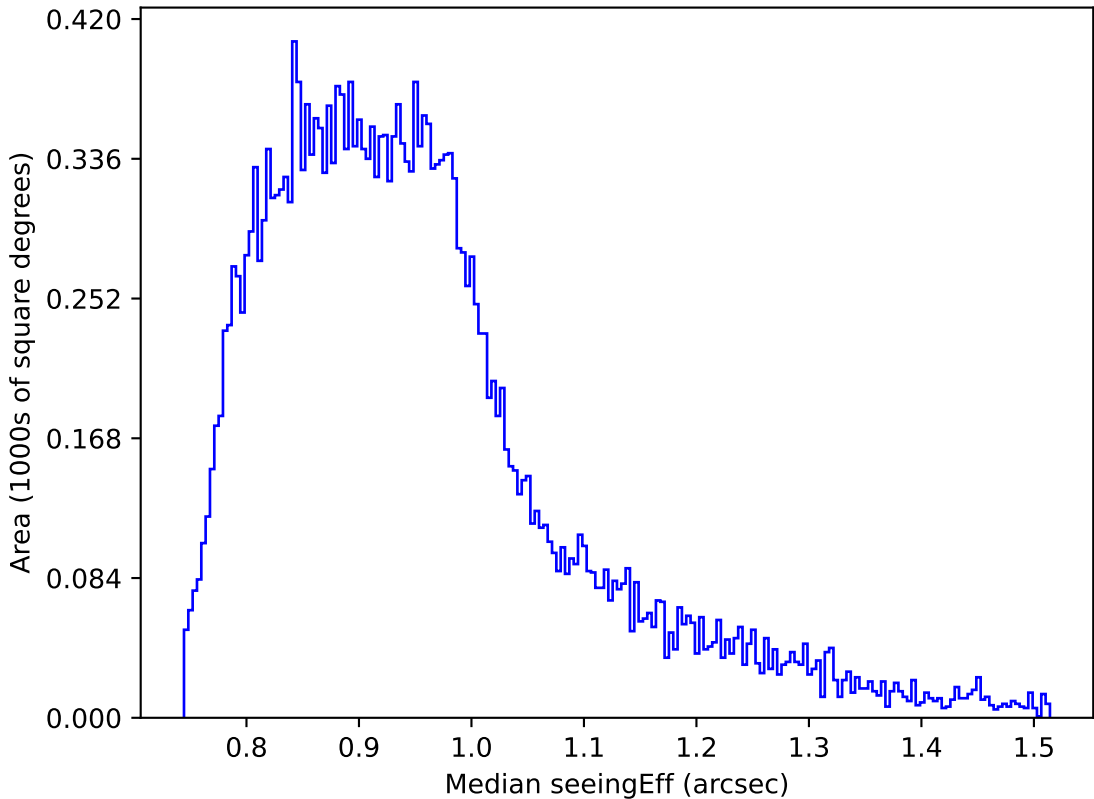
ddf_loaded_half_fl2_v3.4_10yrs Yr 1 i band: Median seeingEff
