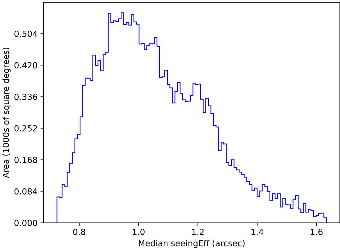
ddf_loaded_half_fI2_v3.4_10yrs Yr 1 g band: Median seeingEff
