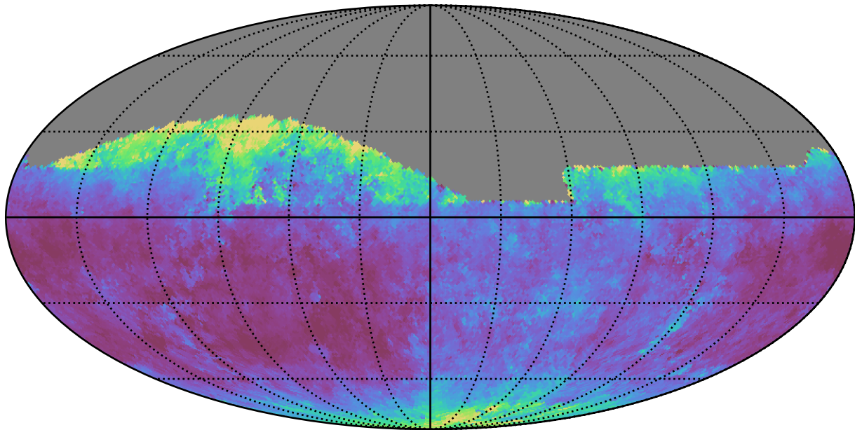
ddf_loaded_half_fl2_v3.4_10yrs Yr 1 all bands: Median seeingEff
