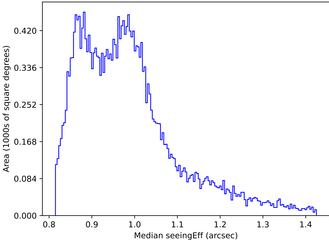
ddf_loaded_half_fl2_v3.4_10yrs Yr 1 all bands: Median seeingEff
