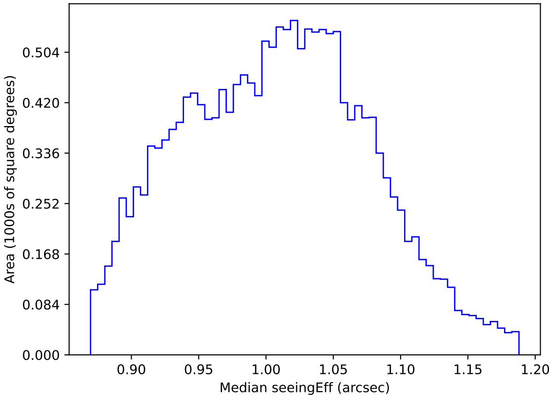
ddf_loaded_half_fl2_v3.4_10yrs WFD z band: Median seeingEff
