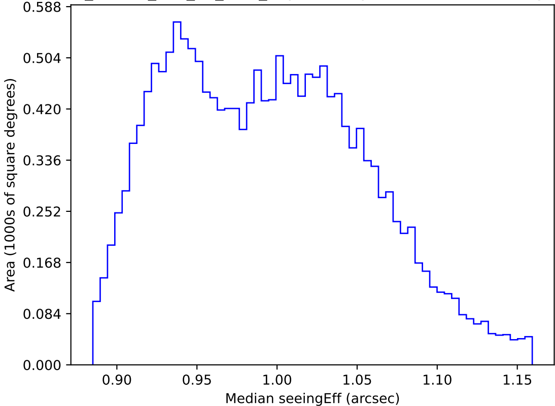
ddf_loaded_half_fl2_v3.4_10yrs WFD y band: Median seeingEff
