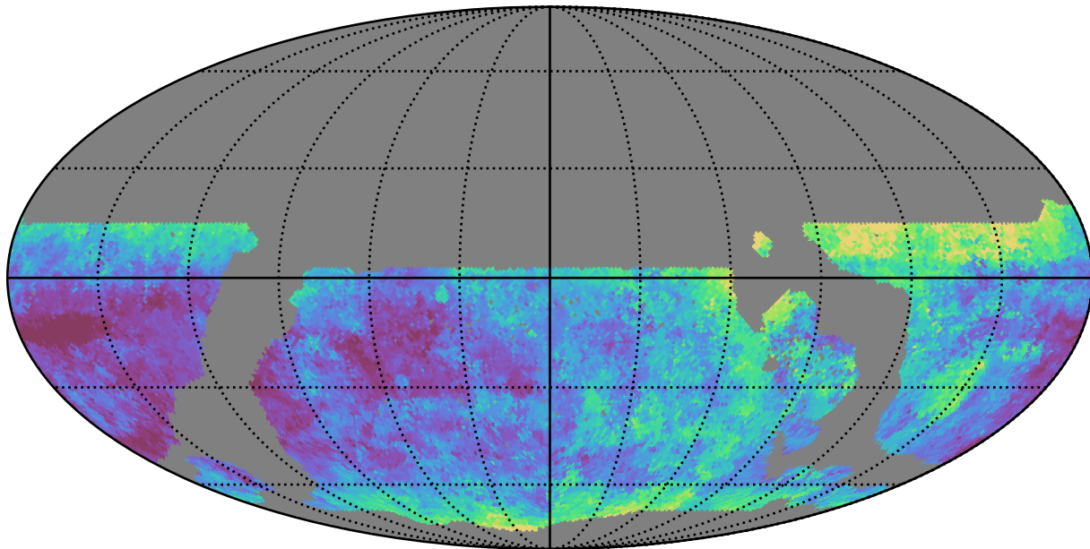
ddf_loaded_half_fl2_v3.4_10yrs WFD u band: Median seeingEff
