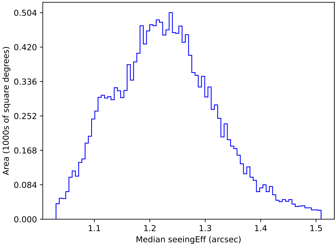
ddf_loaded_half_fl2_v3.4_10yrs WFD u band: Median seeingEff
