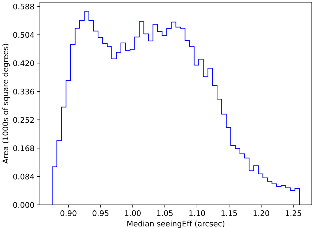
ddf_loaded_half_fl2_v3.4_10yrs WFD r band: Median seeingEff
