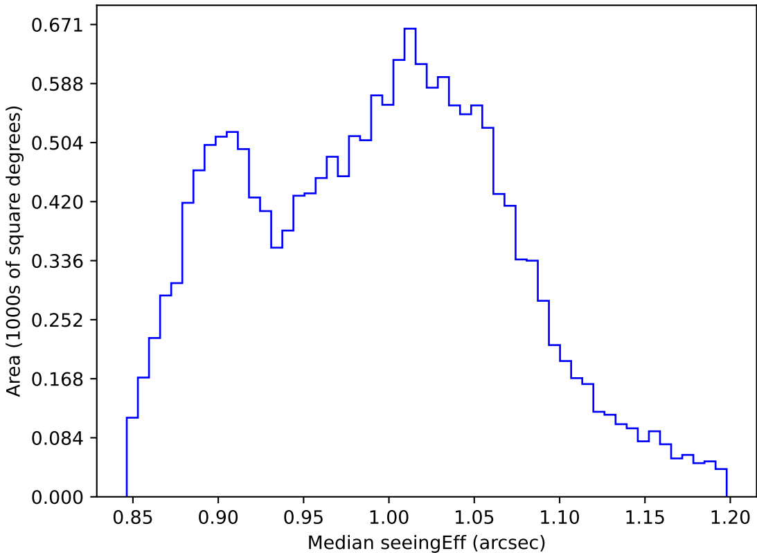
ddf_loaded_half_fl2_v3.4_10yrs WFD i band: Median seeingEff
