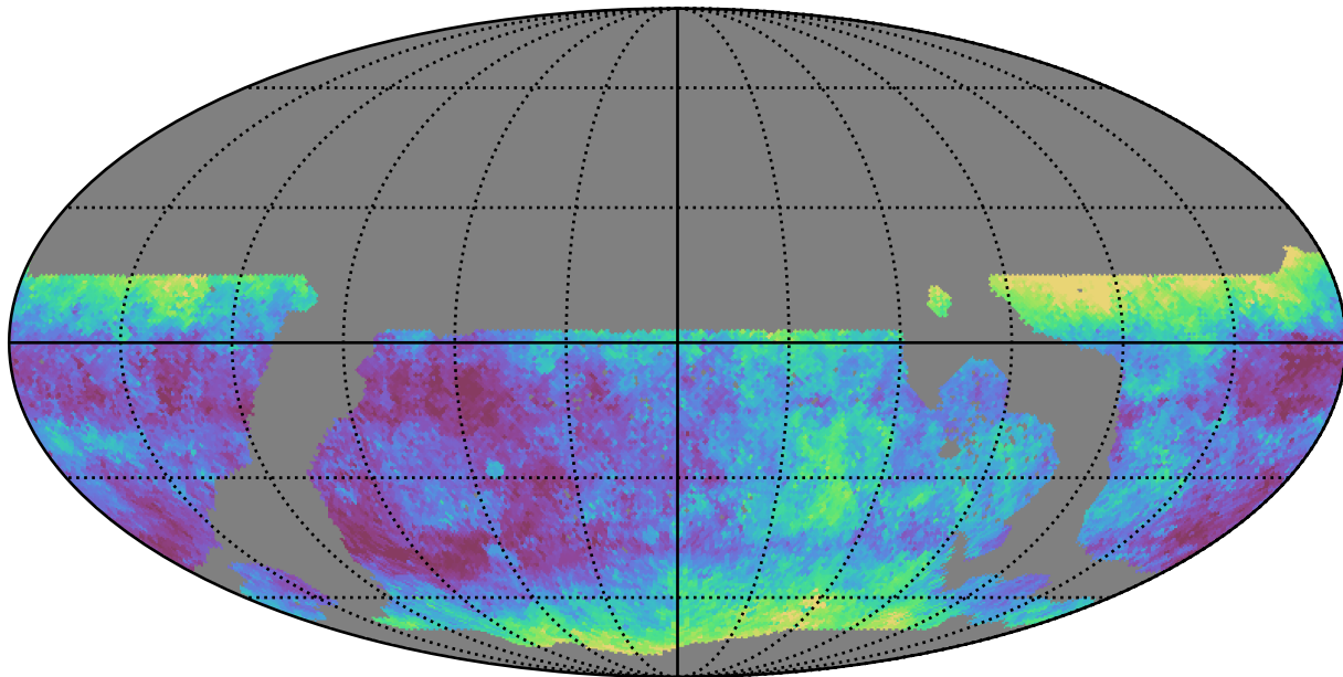
ddf_loaded_half_fl2_v3.4_10yrs WFD g band: Median seeingEff
