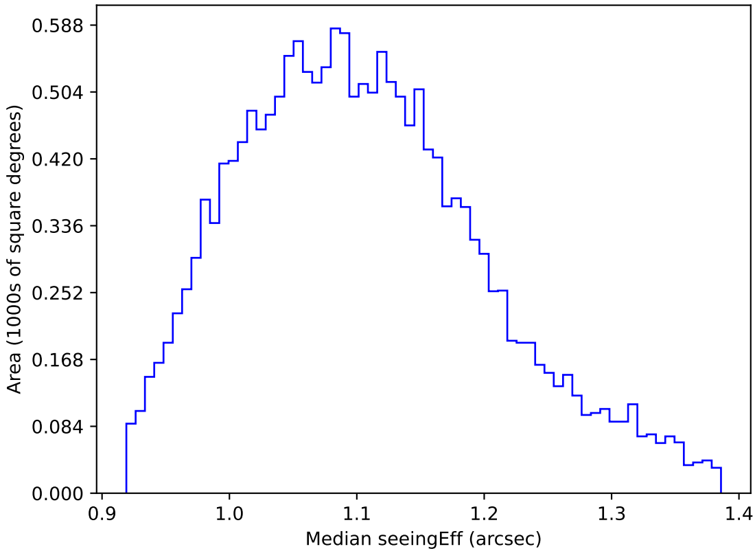
ddf_loaded_half_fl2_v3.4_10yrs WFD g band: Median seeingEff
