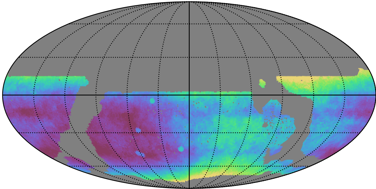
ddf_loaded_half_f12_v3.4_10yrs WFD all bands: Median seeingEff
