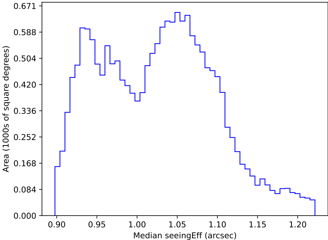
ddf_loaded_half_fl2_v3.4_10yrs WFD all bands: Median seeingEff
