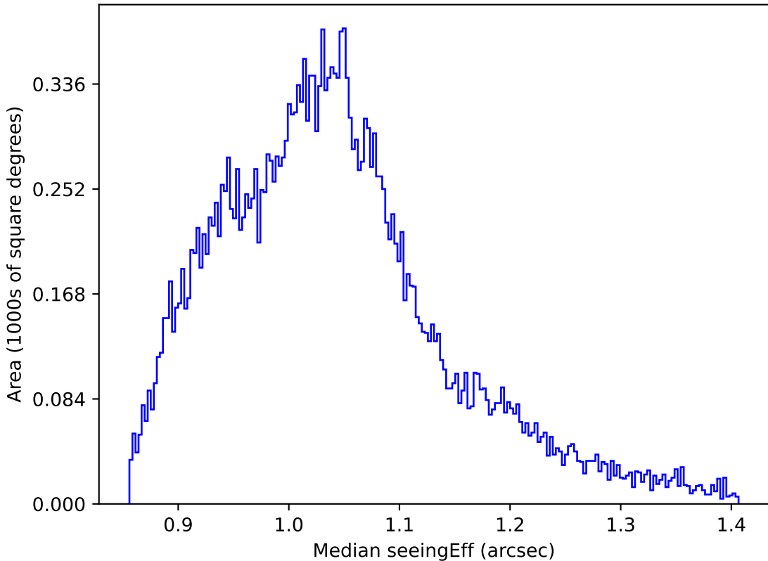
ddf_loaded_half_fl2_v3.4_10yrs All sky z band: Median seeingEff
