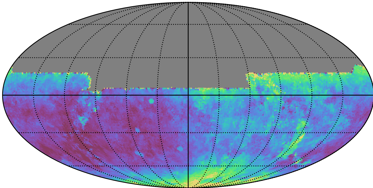
ddf_loaded_half_fl2_v3.4_10yrs All sky y band: Median seeingEff
