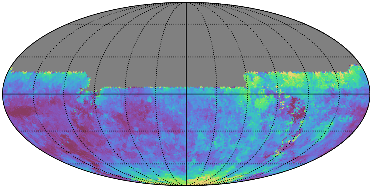
ddf_loaded_half_fl2_v3.4_10yrs All sky u band: Median seeingEff
