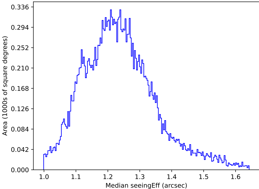
ddf_loaded_half_fl2_v3.4_10yrs All sky u band: Median seeingEff
