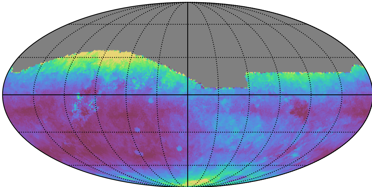
ddf_loaded_half_fl2_v3.4_10yrs All sky r band: Median seeingEff
