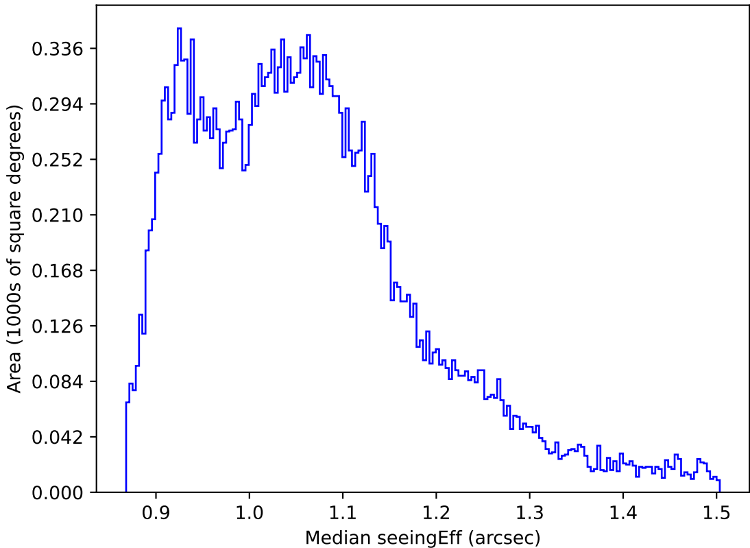
ddf_loaded_half_fl2_v3.4_10yrs All sky r band: Median seeingEff
