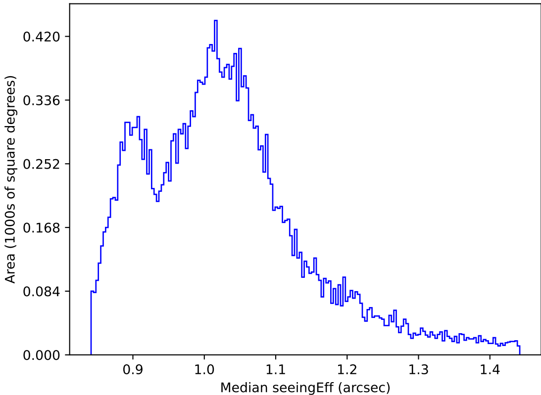
ddf_loaded_half_fl2_v3.4_10yrs All sky i band: Median seeingEff
