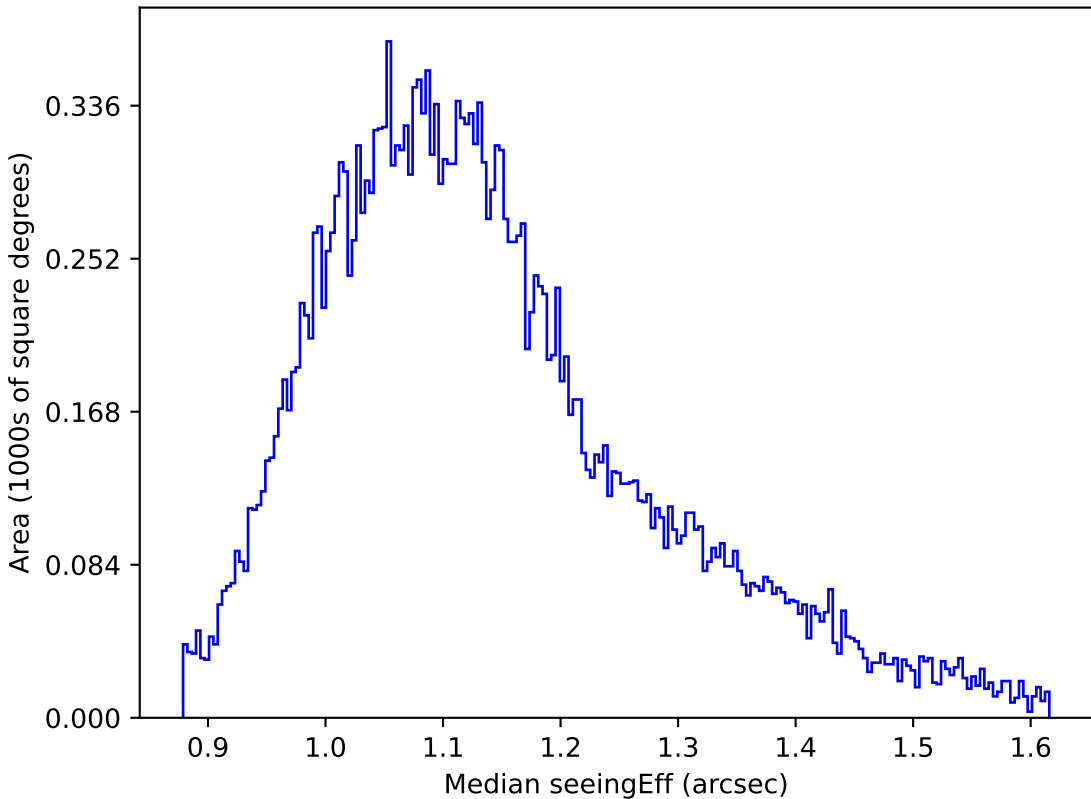
ddf_loaded_half_fl2_v3.4_10yrs All sky g band: Median seeingEff
