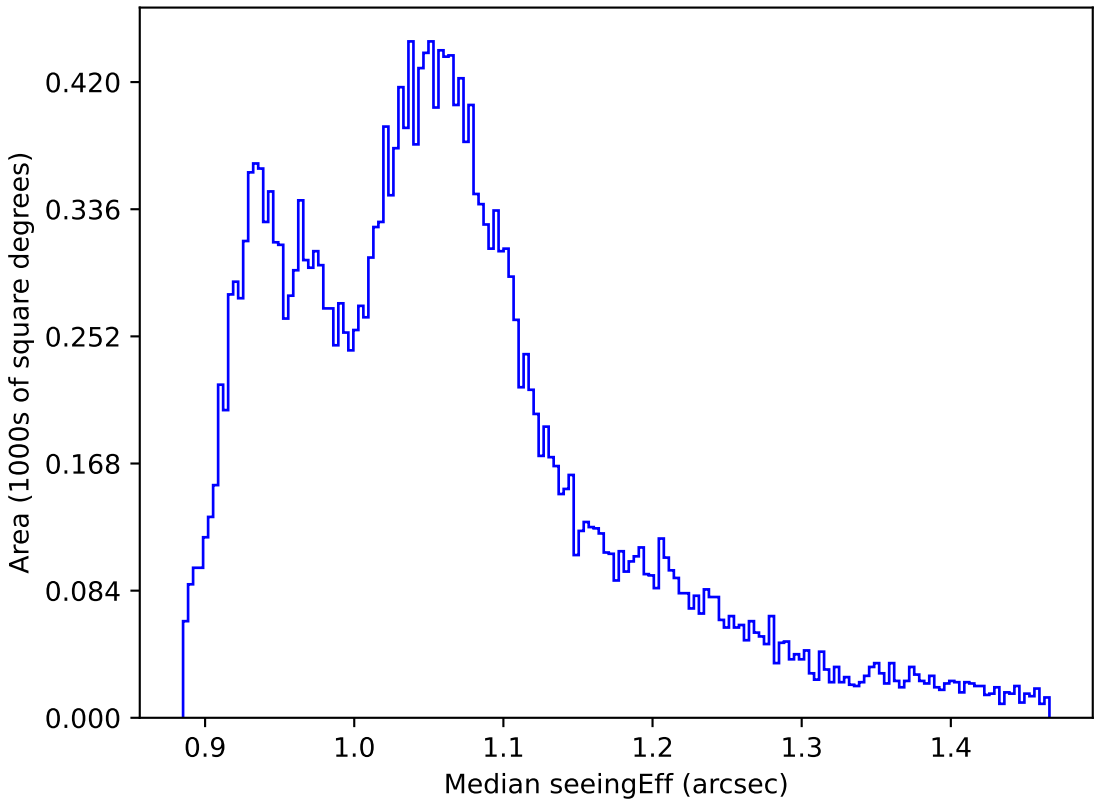
ddf_loaded_half_f12_v3.4_10yrs All sky all bands: Median seeingEff
