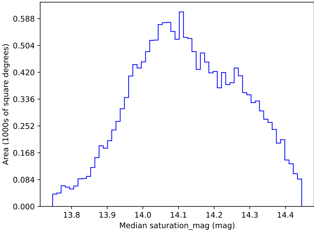
ddf_loaded_half_fl2_v3.4_10yrs WFD z band: Median saturation_mag
