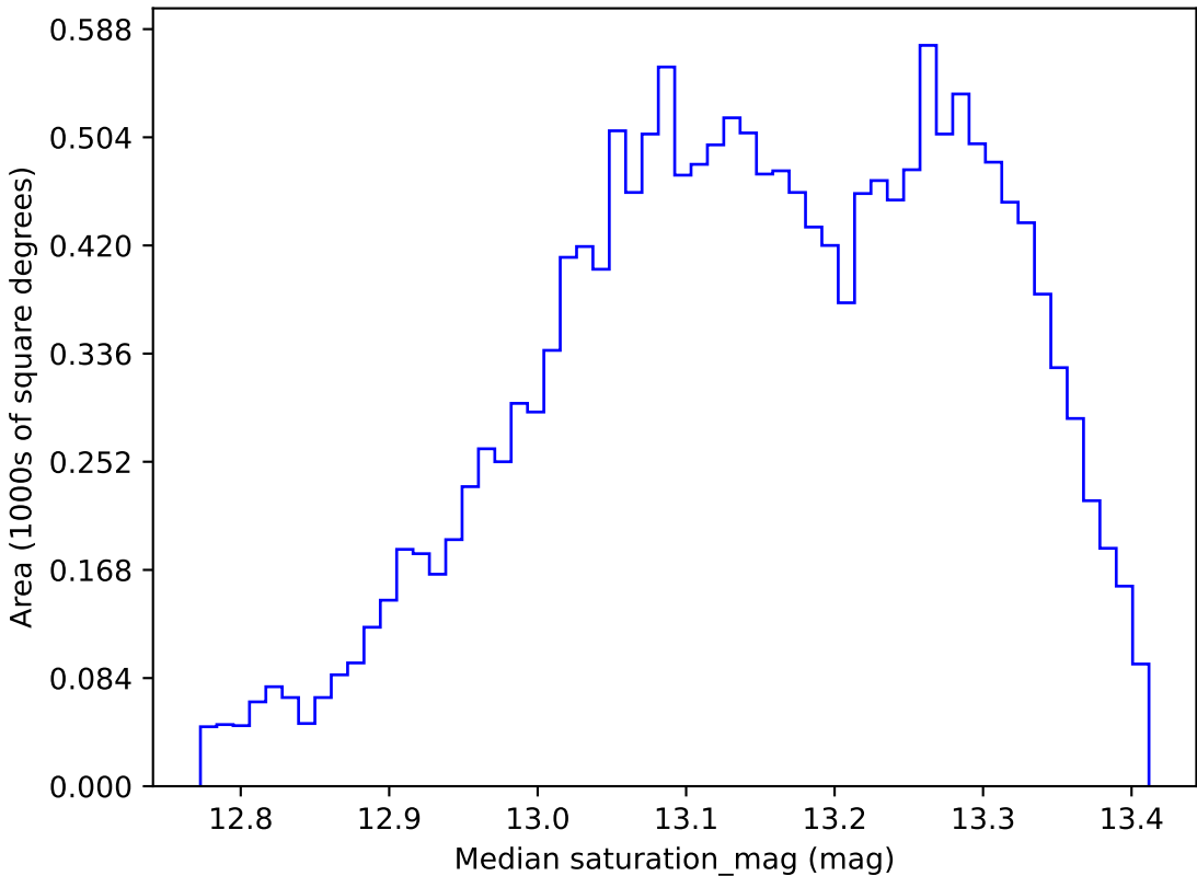
ddf_loaded_half_fl2_v3.4_10yrs WFD y band: Median saturation_mag
