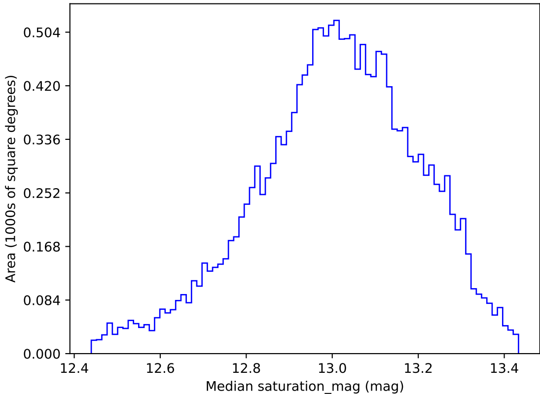
ddf_loaded_half_fl2_v3.4_10yrs WFD u band: Median saturation_mag
