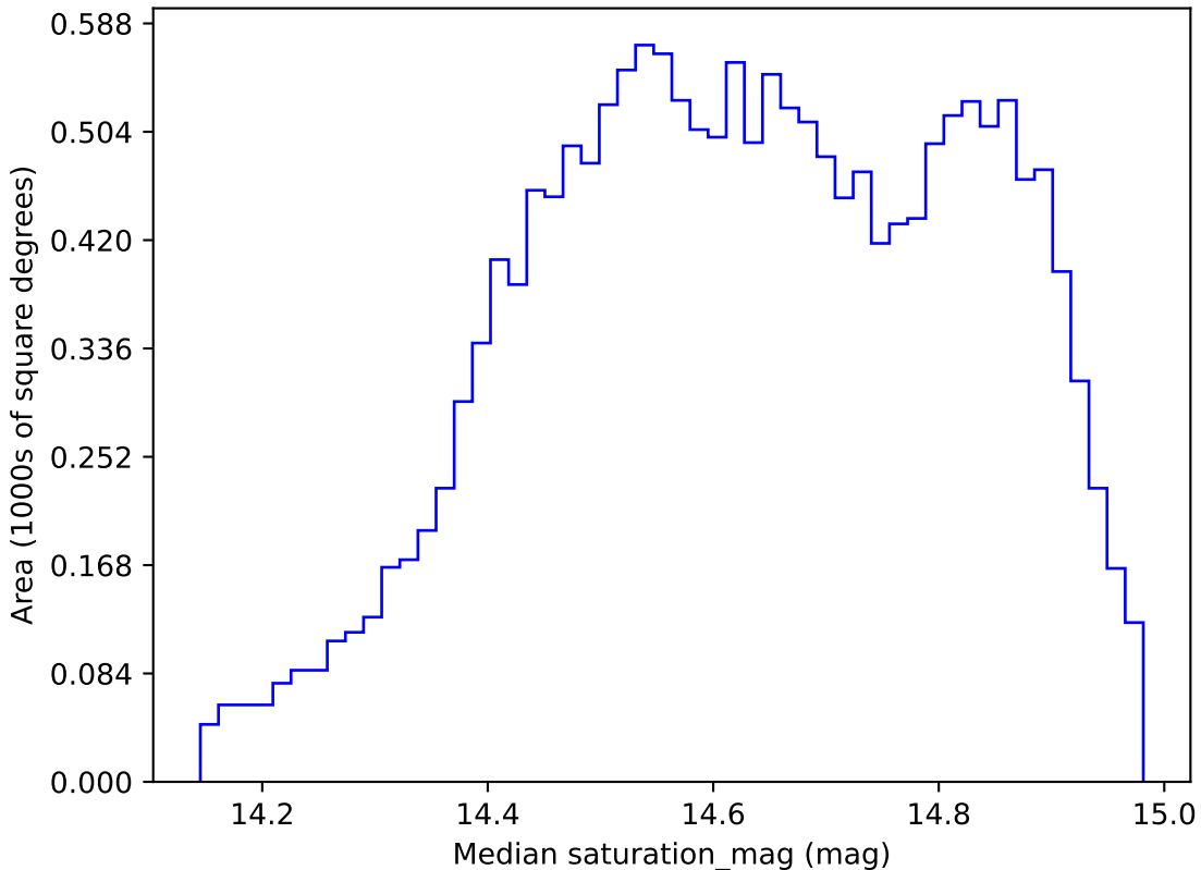
ddf_loaded_half_fl2_v3.4_10yrs WFD r band: Median saturation_mag
