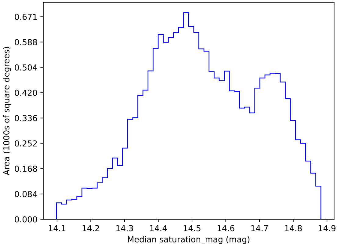
ddf_loaded_half_fl2_v3.4_10yrs WFD i band: Median saturation_mag
