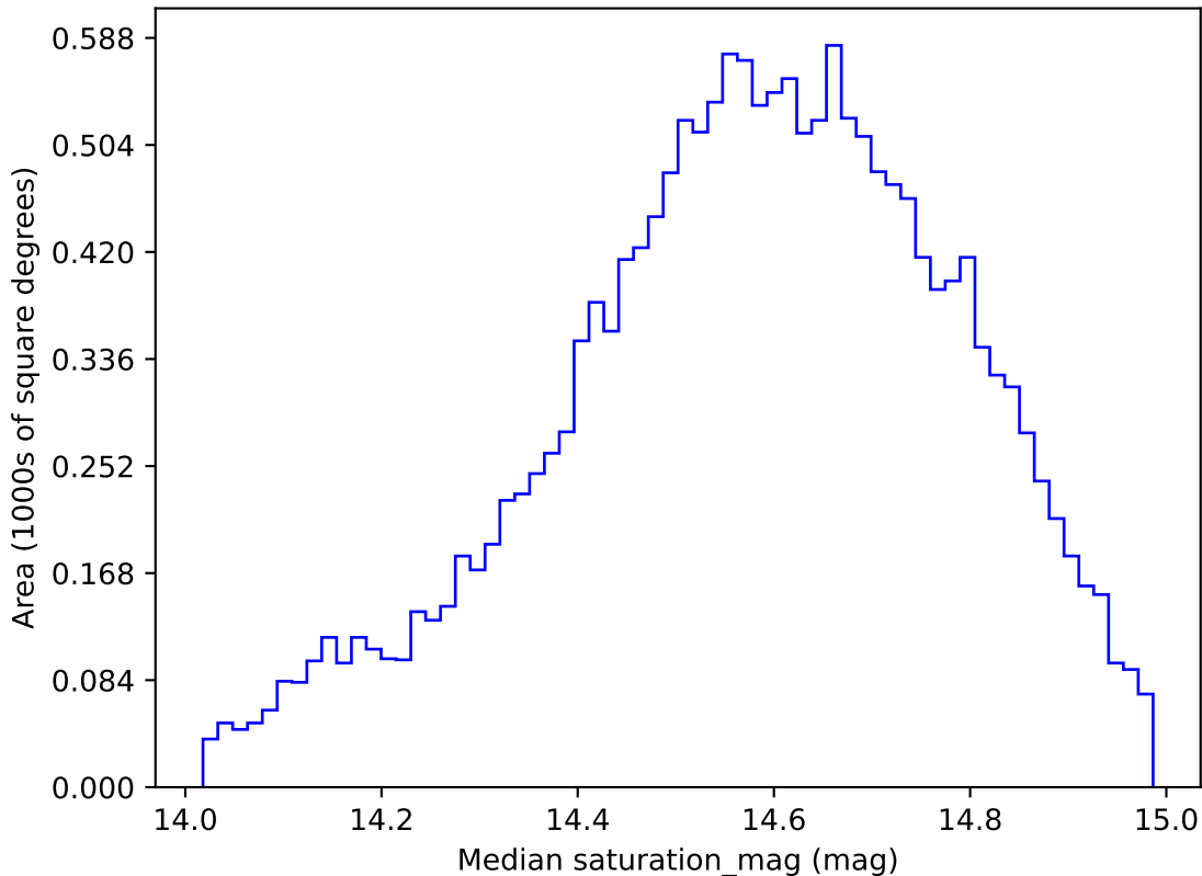
ddf_loaded_half_fl2_v3.4_10yrs WFD g band: Median saturation_mag
