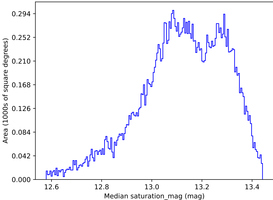
ddf_loaded_half_fl2_v3.4_10yrs All sky y band: Median saturation_mag
