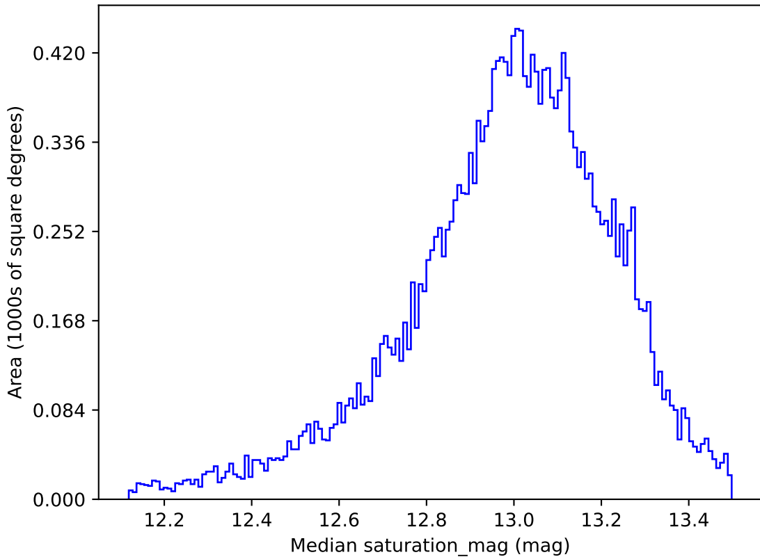
ddf_loaded_half_fl2_v3.4_10yrs All sky u band: Median saturation_mag
